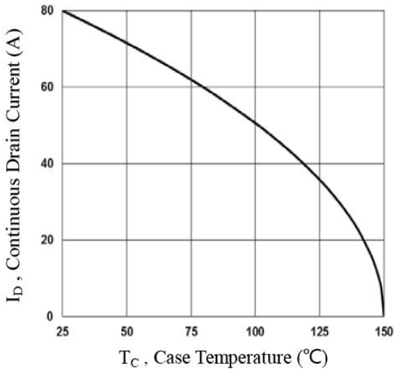
图 1 漏极电流与壳温关系曲线 Fig.1 Continuous Drain Current vs. Tc
