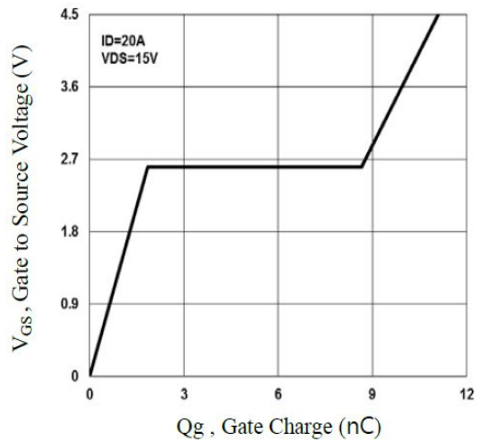
图 4 栅电荷波形 Fig.4 Gate Charge Waveform
