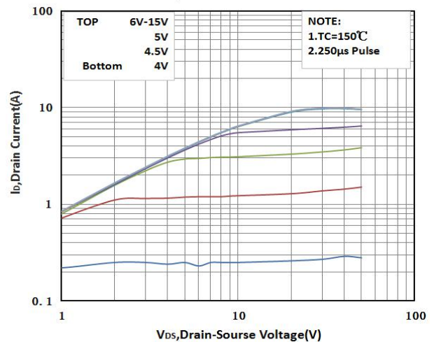
图 4 输出特性曲线, Tc=150°C Fig4 Typical Output Characteristics
