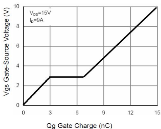
Figure 5 Gate Charge
