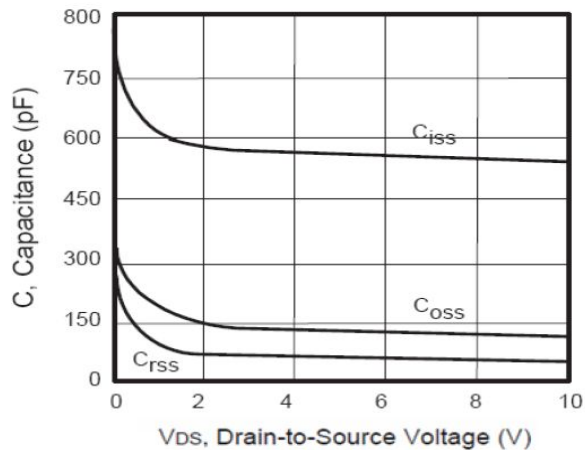
Figure 4 Capacitance
