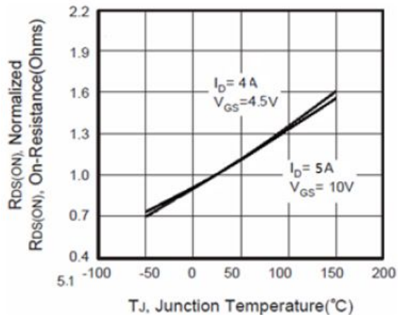
Figure 3 Rdson & Tj
