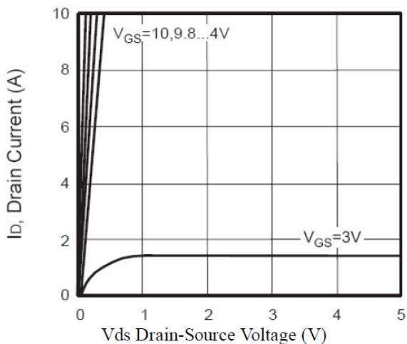
Figure 1 output characteristic
