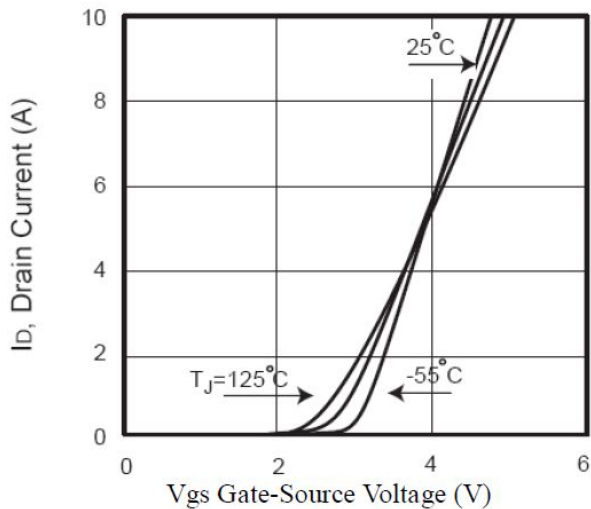
Figure 2 Transfer characteristic
