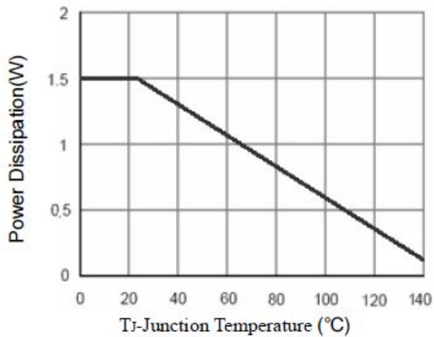
Figure 6 Power Dissipation
