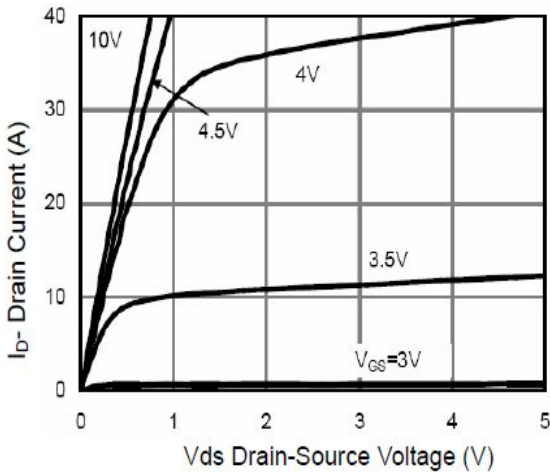
Figure 1: output characteristic 图 1 输出特性曲线, T_c=25^\circ\text{C}
