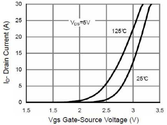
Figure 2: transfer characteristic 图 2 转移特性曲线
