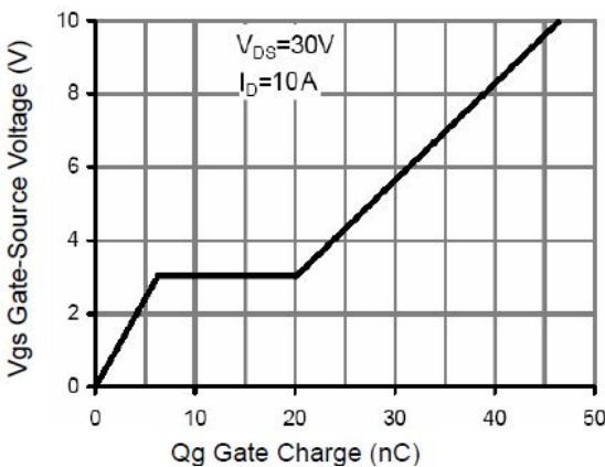
Figure 5: Gate Charge 图 5 典型栅极电荷与栅源电压曲线
