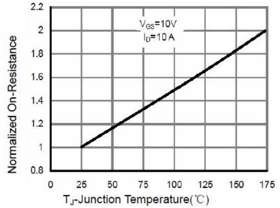
Figure 4: R_{DS(on)} -Junction temperature 图 4 导通电阻与结温度曲线
