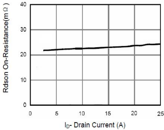
Figure 3: Resistance & I_D 图 3 导通电阻与漏极电流曲线
