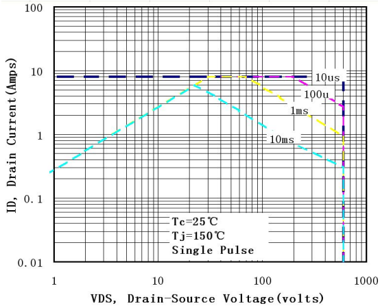
图 6-1 SIF2N60C(TO-220)
