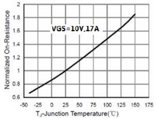
Figure 4 Rdson-Junction Temperature
