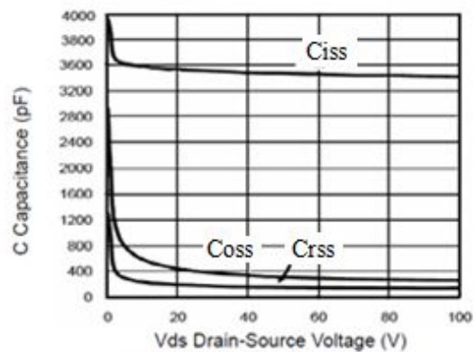
Figure 6 Capacitance vs Vds
