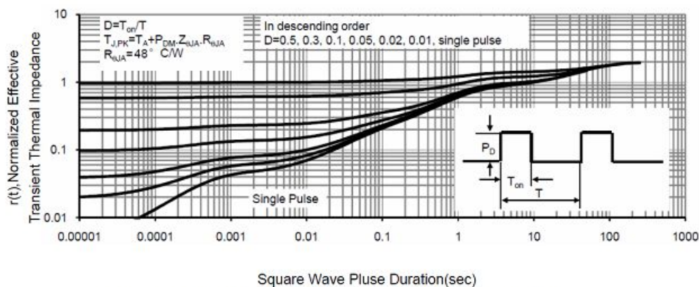
Figure 10 Normalized Maximum Transient Thermal Impedance
