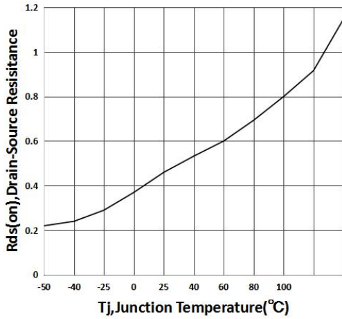
图 3 导通电阻与温度曲线 Fig3 Normalized On-Resistance Vs. Temperature
