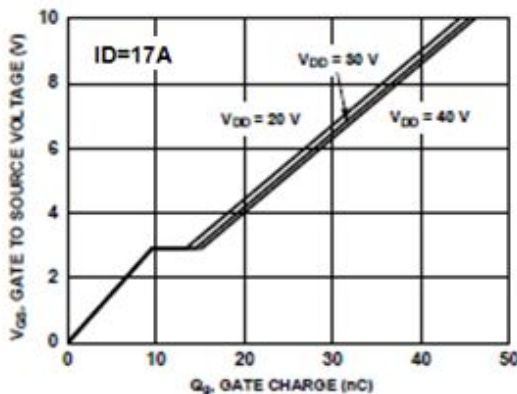
Figure 5 Gate Charge
