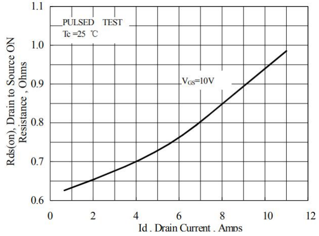
图 2 导通电阻与漏极电流和栅极电压曲线 Fig2 On-Resistance Vs.Drain Current and Gate Voltage
