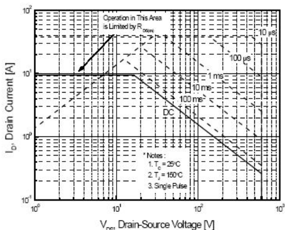
Fig6-3 Maximum Safe Operating Area
